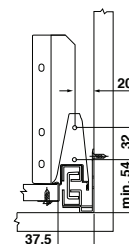
Front drilling dimensions
