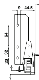
Back drilling dimensions
