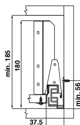
Cabinet drilling dimensions
